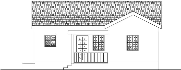
FRONT ELEVATION
